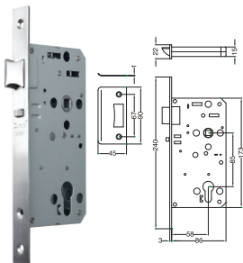
DR-ML85 Mortise Classroom Lockcase Backset : 60 x 85 mm
